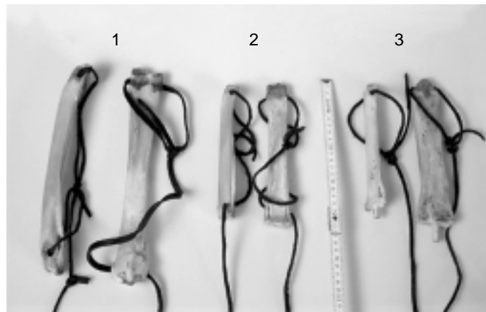
Fig. 8. Finished bone skate replicas (Photo: H. Ch. Küchelmann).
